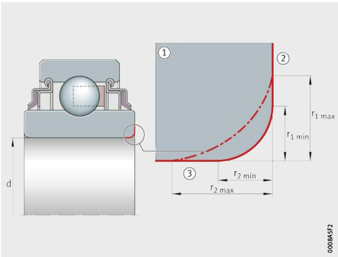
Figure 9 Symmetrical ring cross-section with identical chamfer dimensions on both rings
