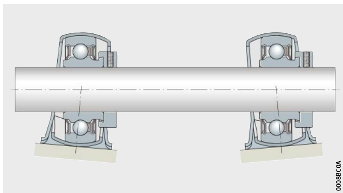
Figure 5 Compensation of static housing misalignment
