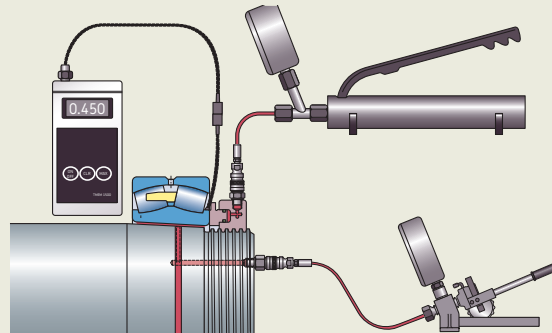
Mounting with SKF SensorMount
