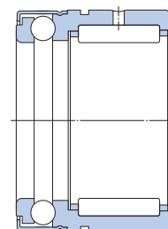
NX..Z ( F_w \geq 10 mm)
