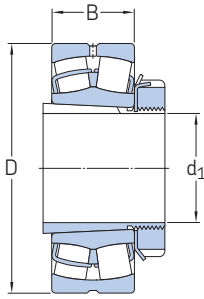
Bearing on an H .. sleeve
