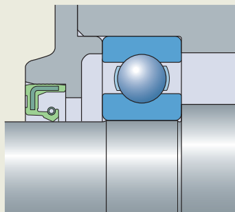
Fig. 14 Radial shaft seal, mounted for lubricant retention
