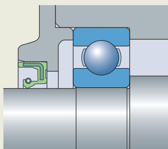
Fig. 15 Radial shaft seal, mounted for contaminant exclusion
