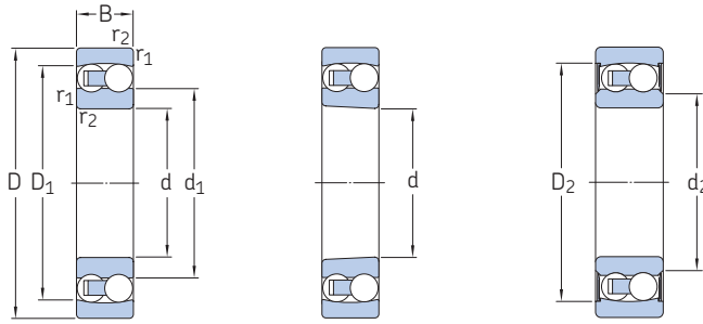
Cylindrical bore
